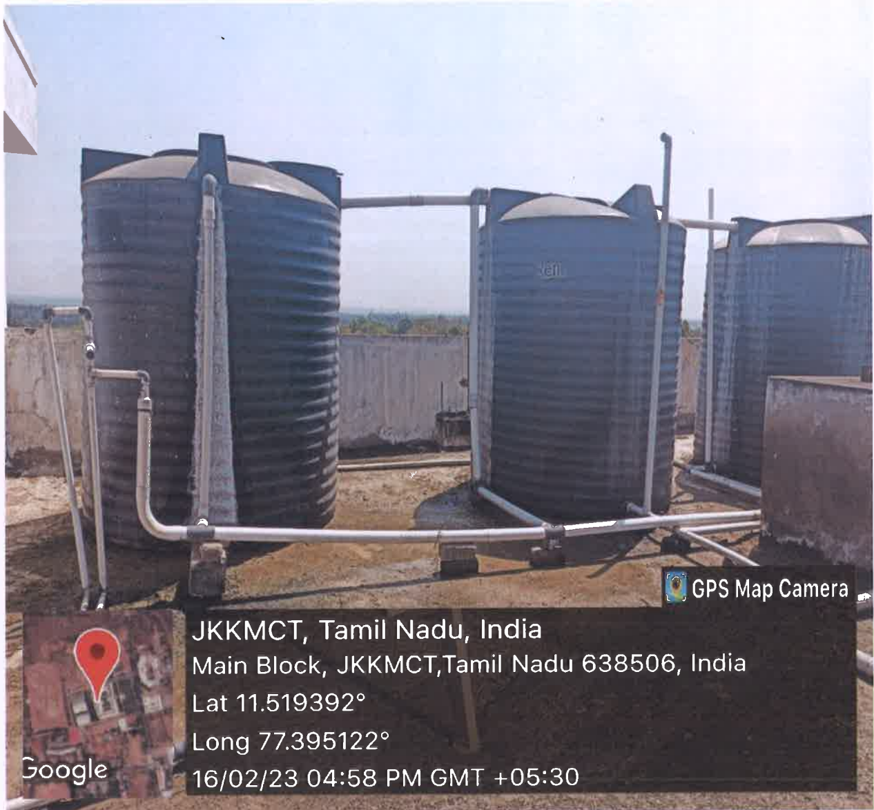
Photos of One Pipe System
